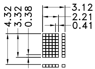
DOT DETAIL SCALE 2:1
