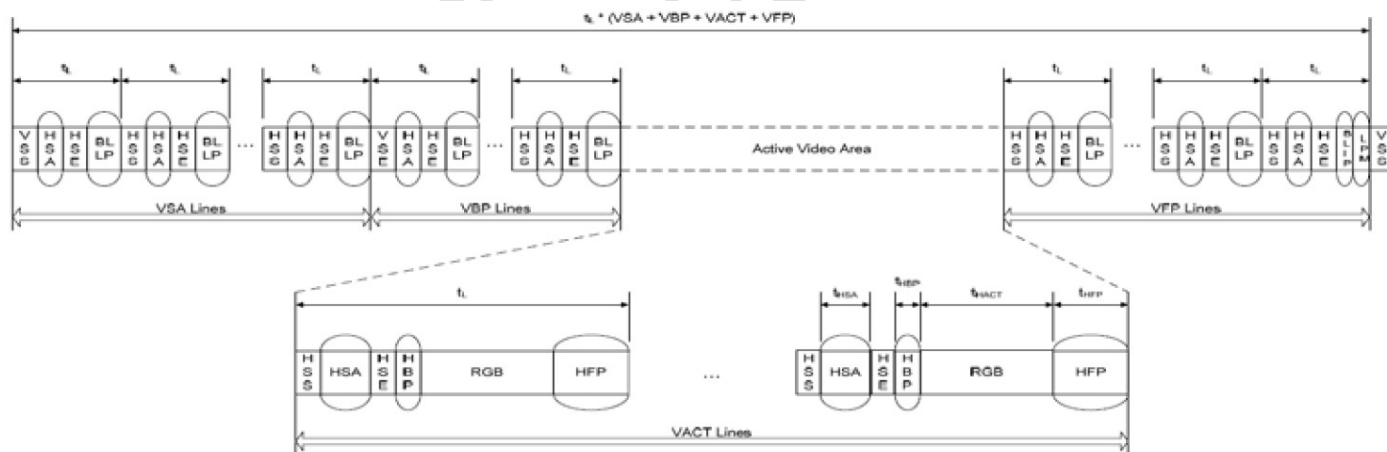
Figure 9-1 Non-Burst Mode with Sync Pulses
