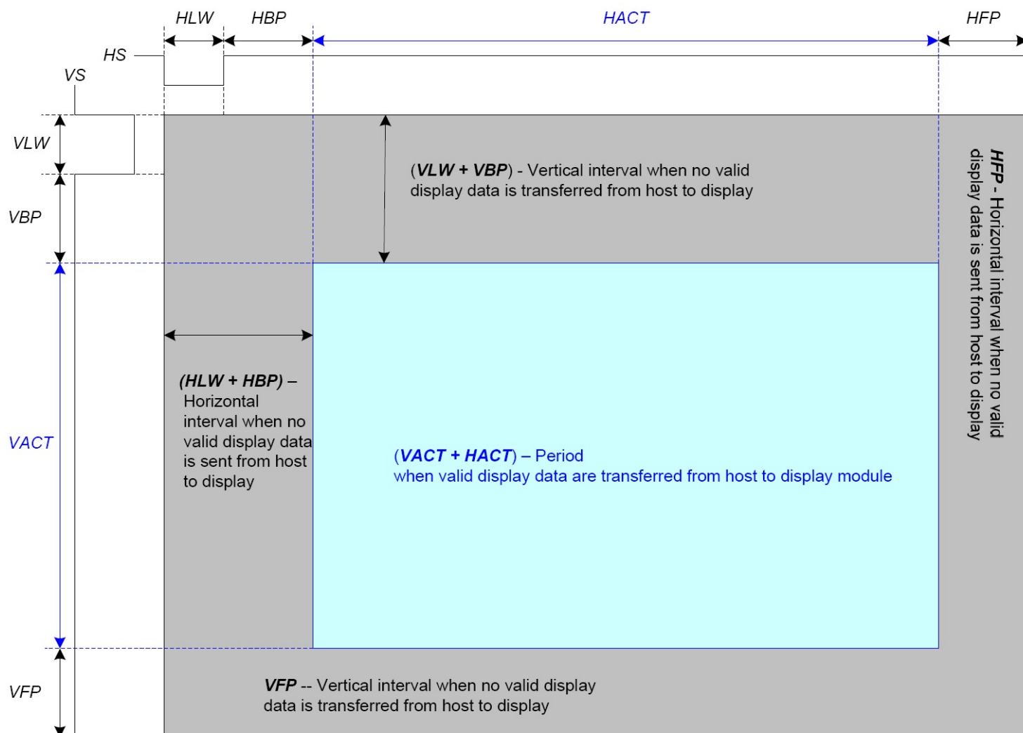
Figure 7-1 DRAM Access Area by RGB Interface
