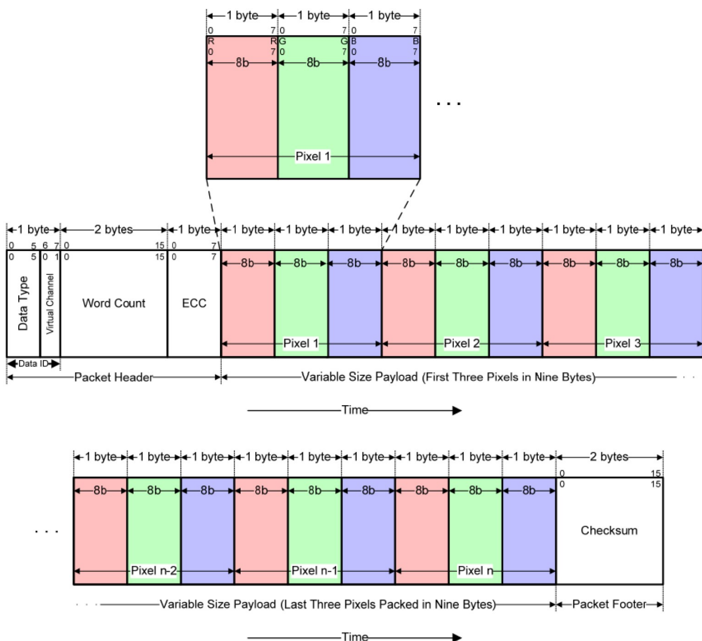
Figure 6-1 DSI RGB888 (24bpp) Color format, Long Packet
