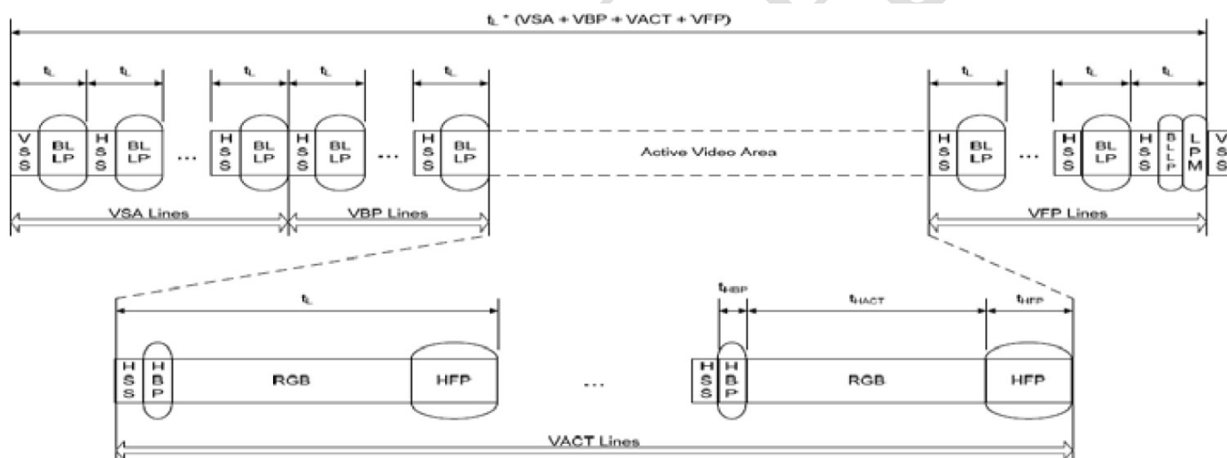
Figure 9-3 Burst mode
